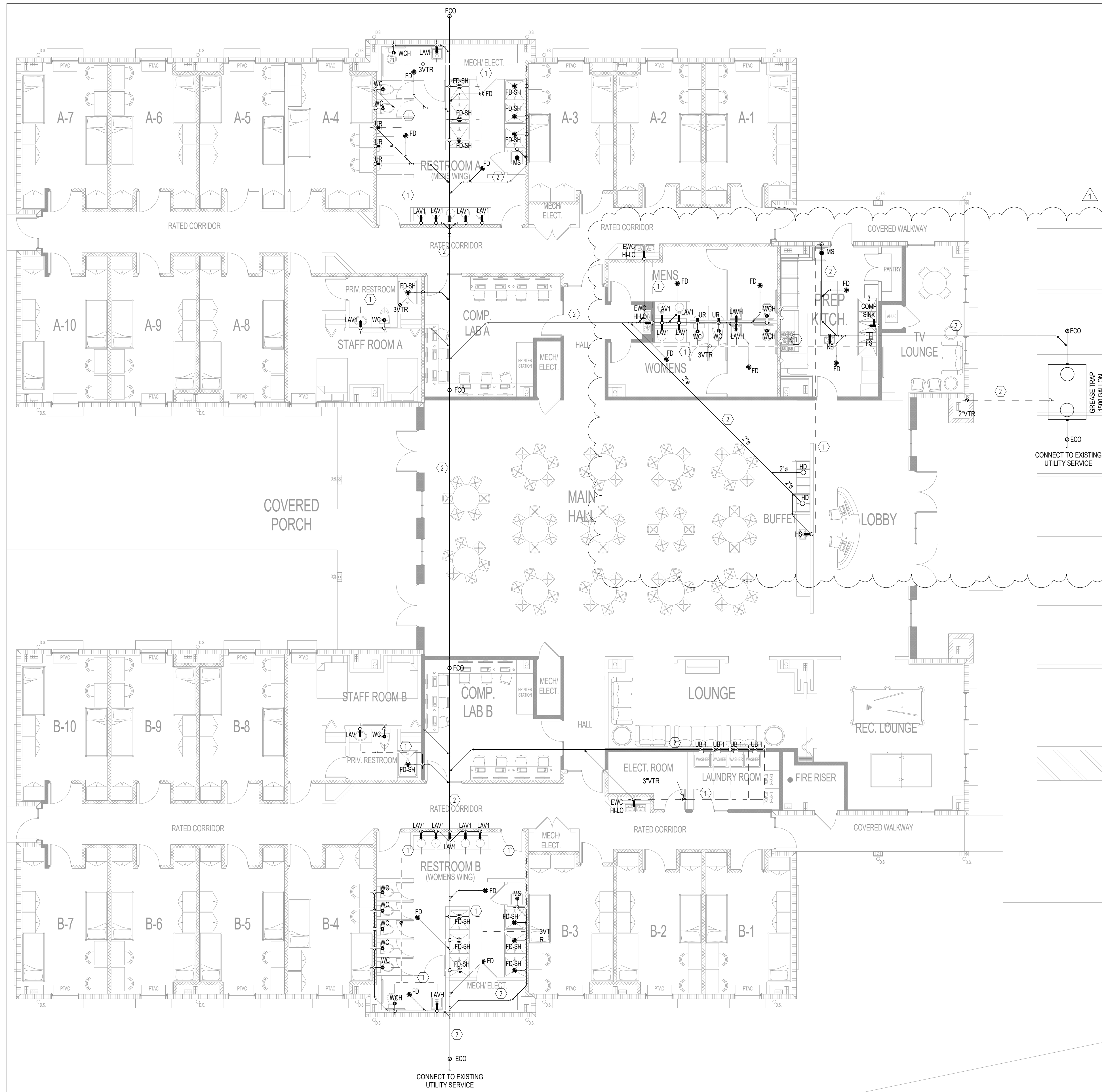
1 Plumbing Floor Plan Sewer - Line P-1 1/8" = 1'-0"
