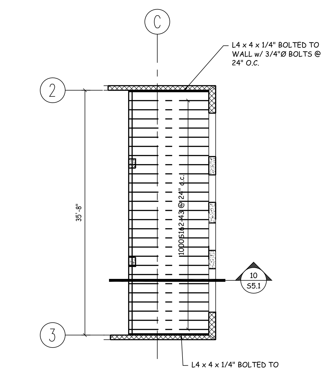
SHED ROOF FRAMING PLAN ② SCALE: 1/8" = 1'-0"
