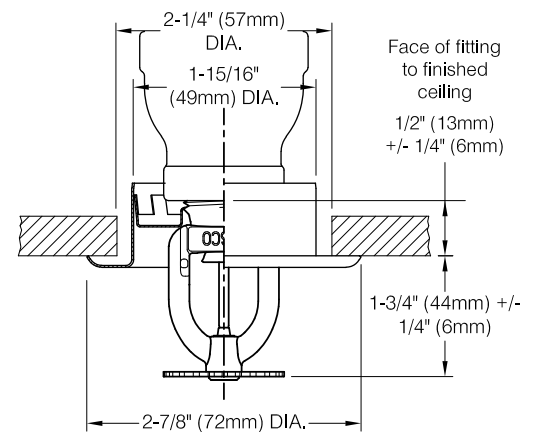
F2 & FV Recessed Escutcheon Installation
