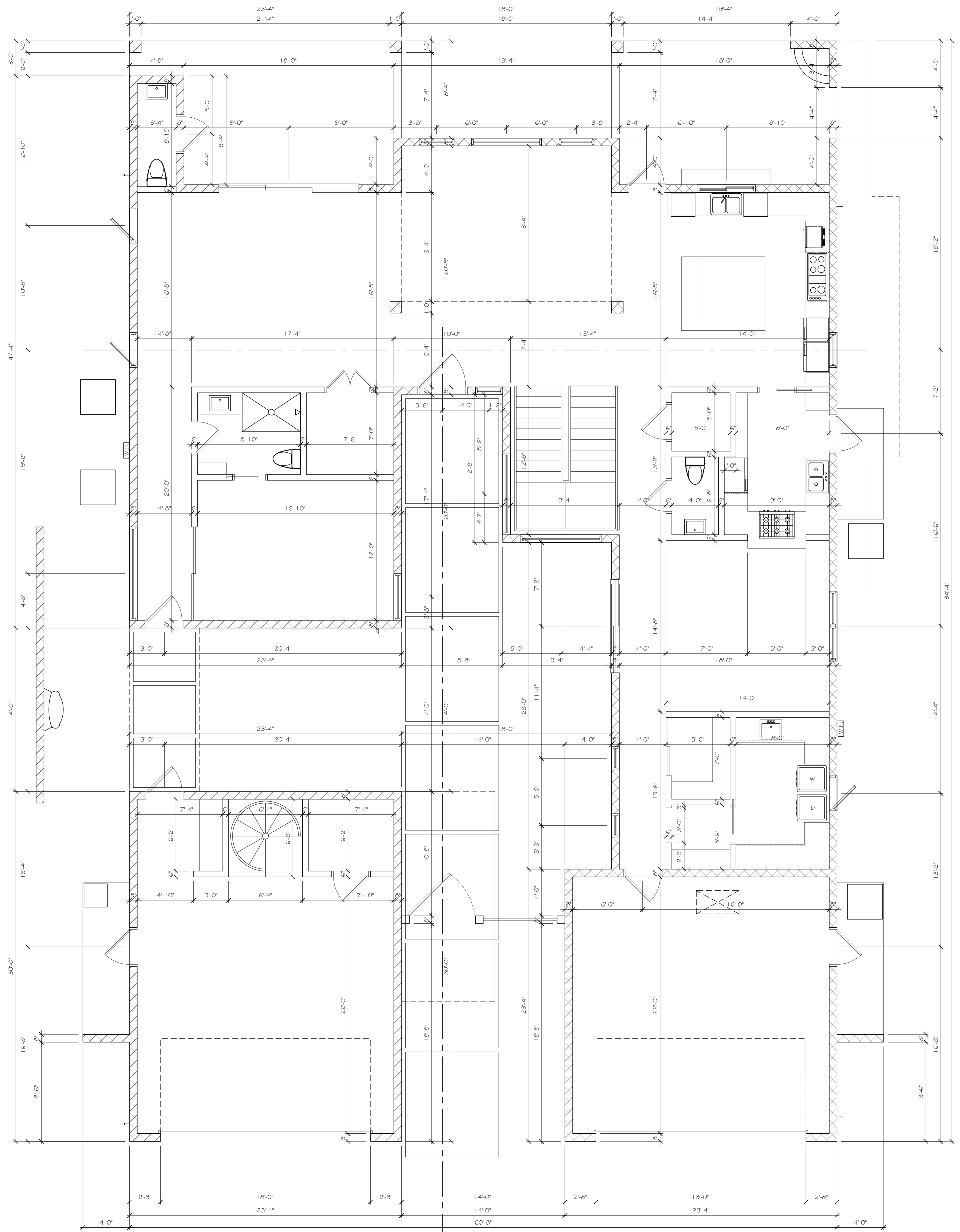
LOWER LEVEL FLOOR PLAN - DIMENSIONED
