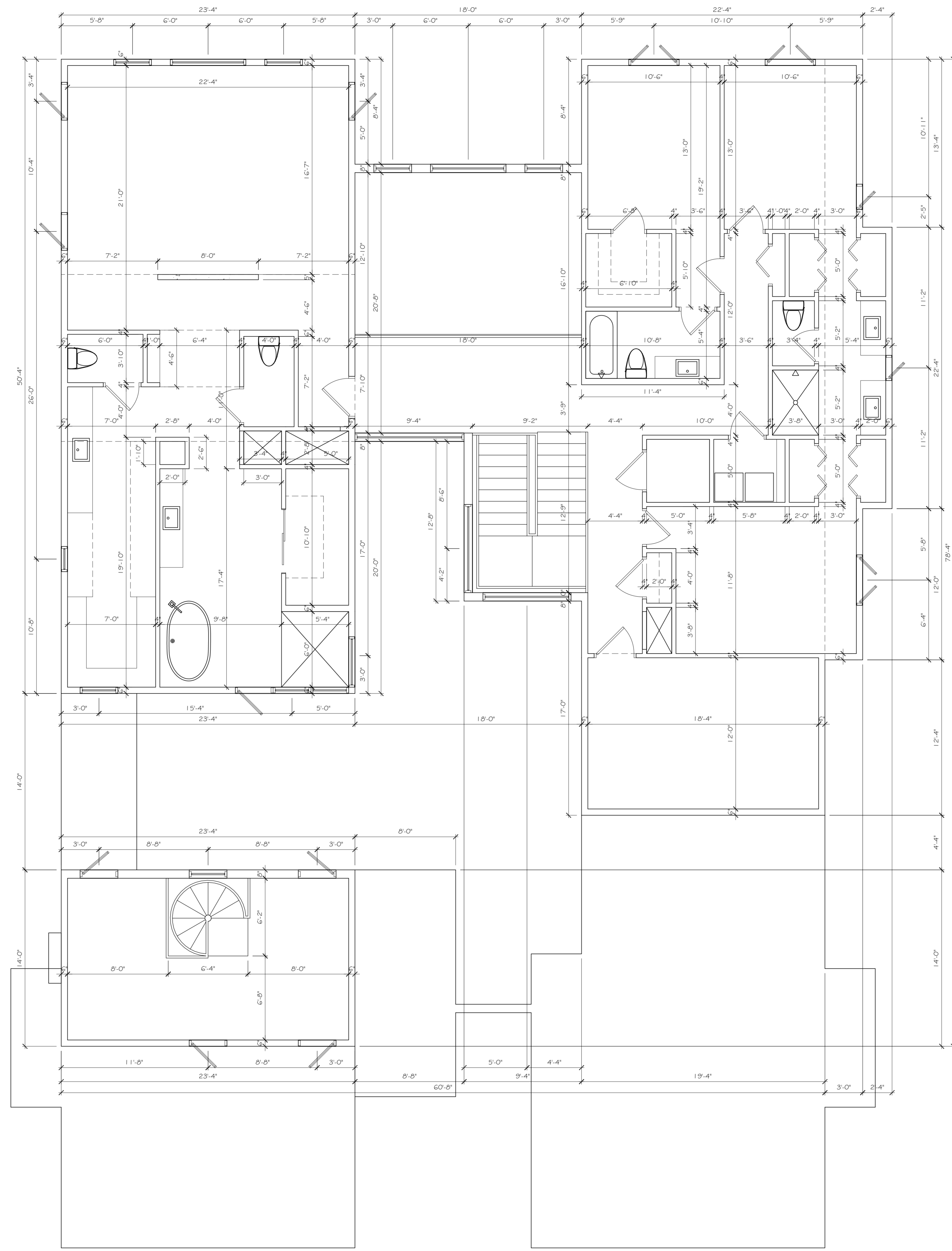
UPPER LEVEL FLOOR PLAN - DIMENSIONED
